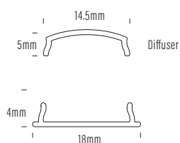
AQS-170-ACC-04 1m Aluminium Profile PMMA Diffuser
