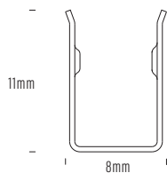
AQS-402-ACC-02 Bendable S Channel
