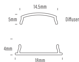
AQS-170-ACC-05 2m Aluminium Profile PMMA Diffuser
