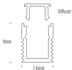
AQS-172-ACC-02 Aluminium Profile PMMA Diffuser
