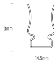
AQS-500-ACC-AL-01-SS 316SS mounting clips
