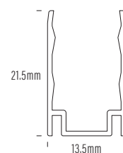
AQS-500-ACC-AL3-02 2m Aluminium
