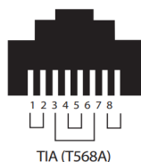
T568A Cabling Pinout Specifications
