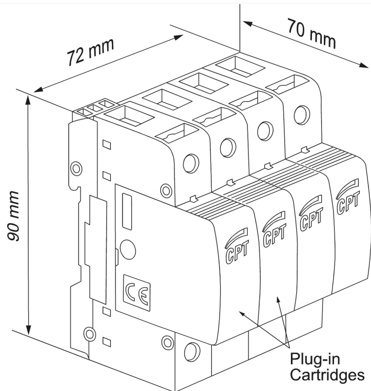
Dimension Diagram
