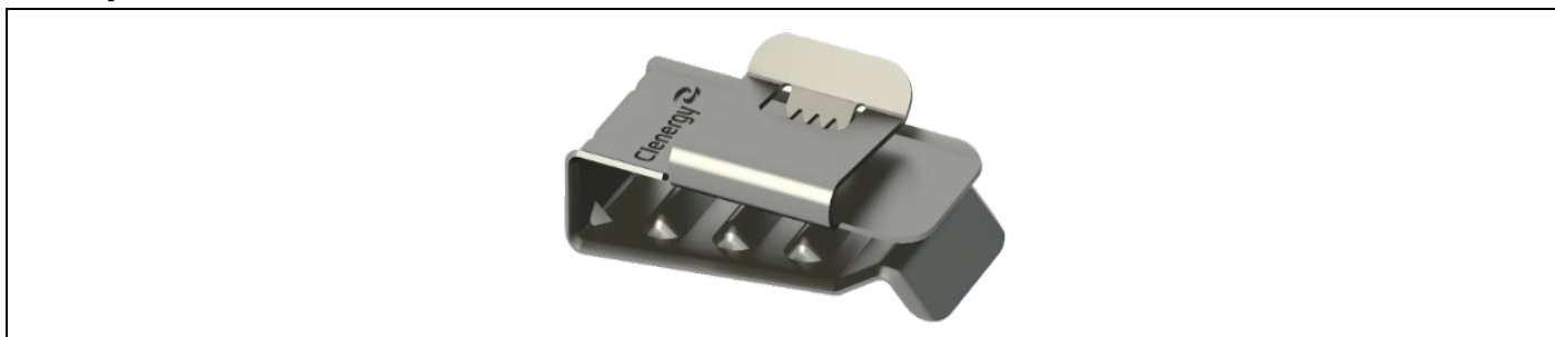
Universal Cable Clip for PV Panels for holding 4 cables, Landscape Part No.: EZ-CC-PV/4/L
