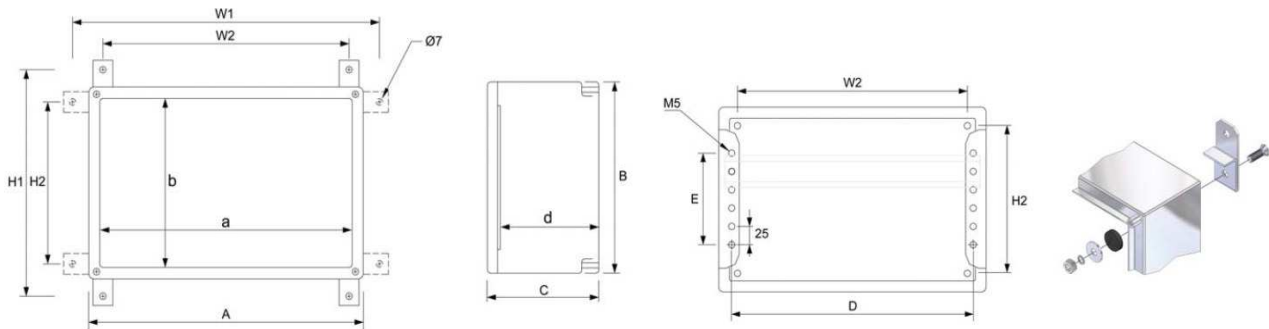
MAIN DIMENSIONS
