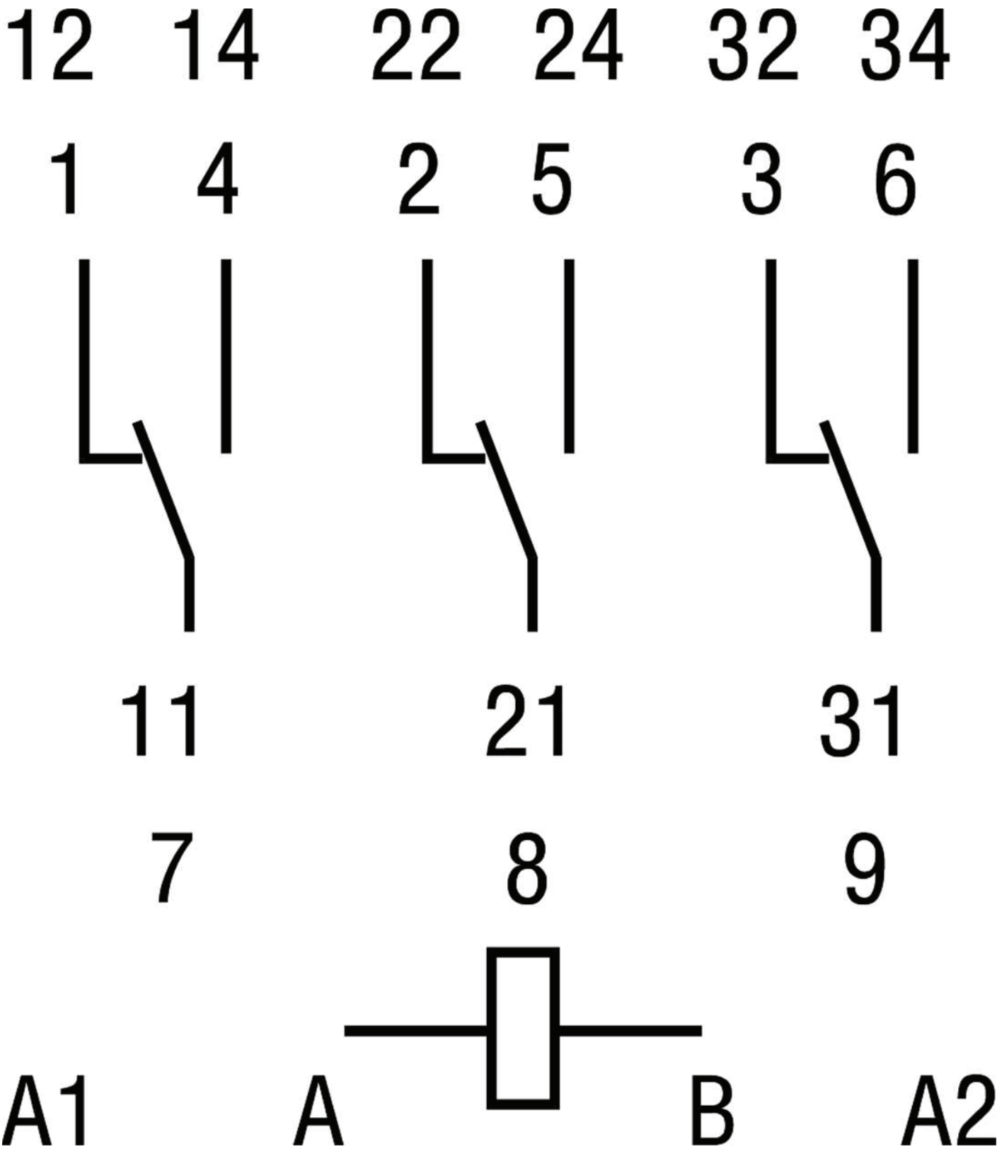
Connection / Wiring Diagram
