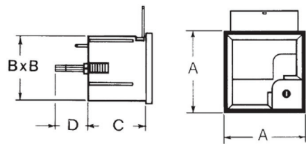
Meter dimensions
