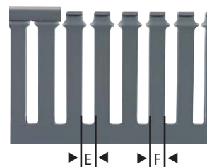
Detail of duct body/cover coupling for maximum wire retention and maximum solidity.
