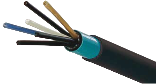
Outdoor Highlight Gel-filled Loosetube Sacrificial Sheath Cable
