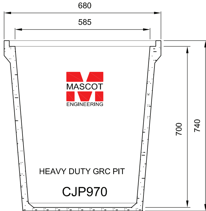
SECTION VIEW
