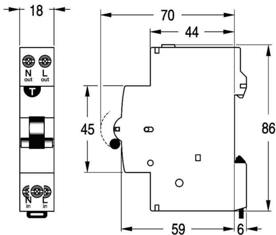
Dimension Diagram
