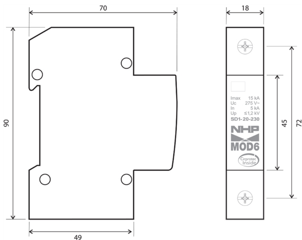
Dimension Diagram
