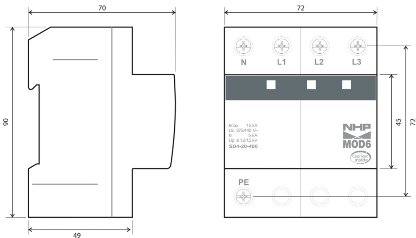
Dimension Diagram
