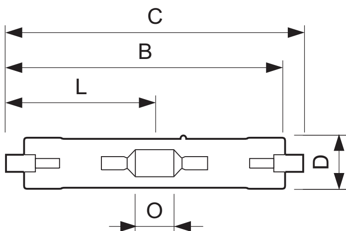
MHN-TD 150W/842 RX7s 1CT
