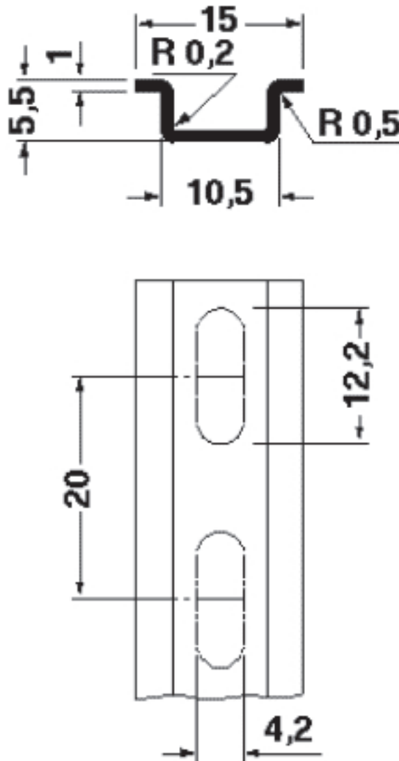
Dimensioned drawing
