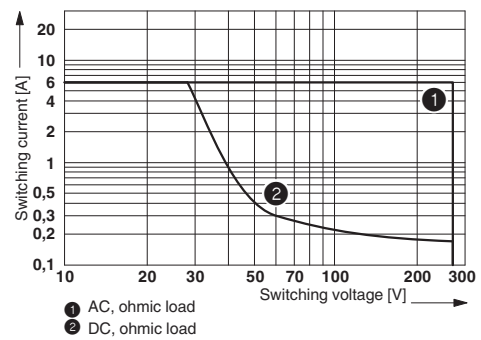
Interrupting rating
