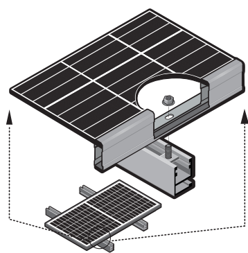
Fig. 17: Mounting hole installation example
