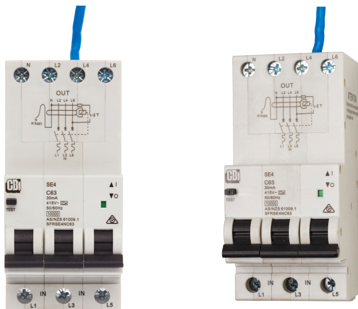
SFRSE4 | Residual Current Operated Circuit Breaker | 3 + N | 10 kA
