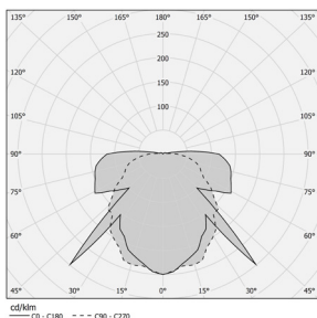
32W LED
