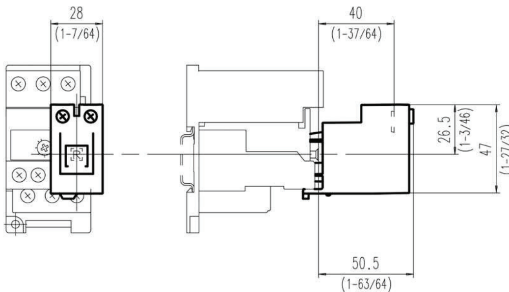
Dimension Diagram
