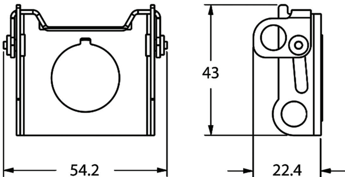
Dimension Diagram
