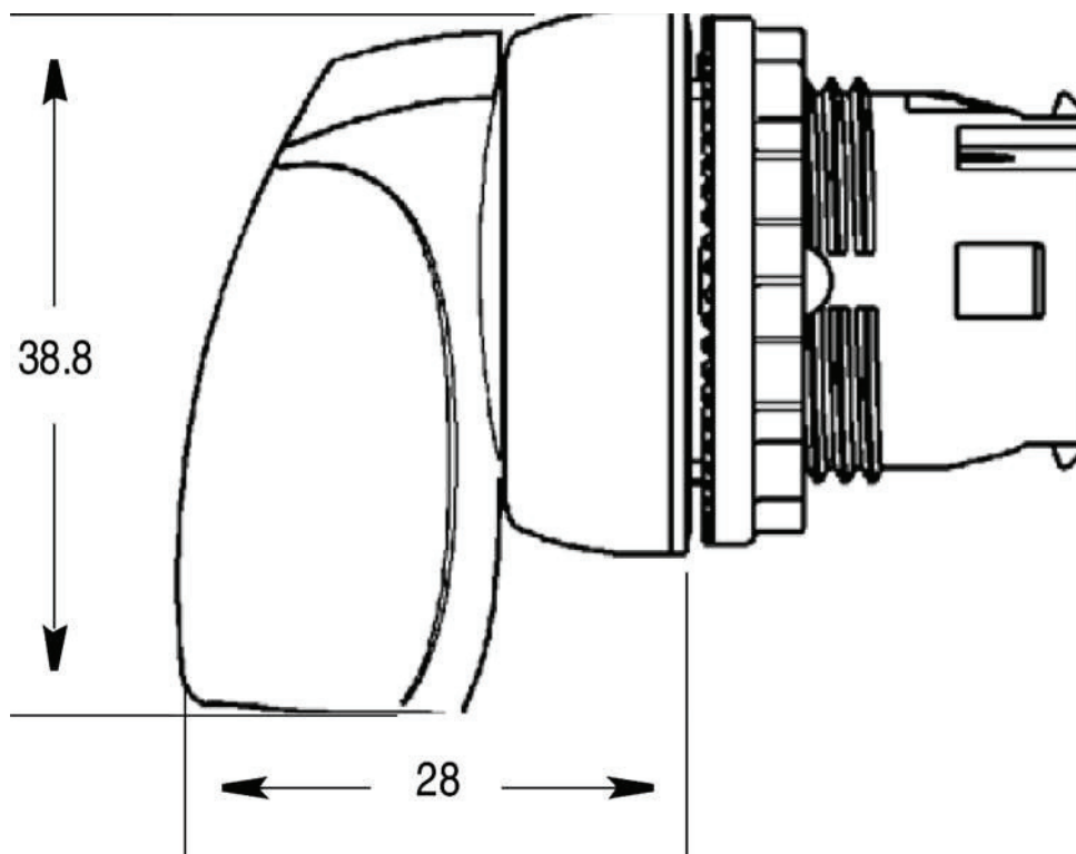
Dimension Diagram
