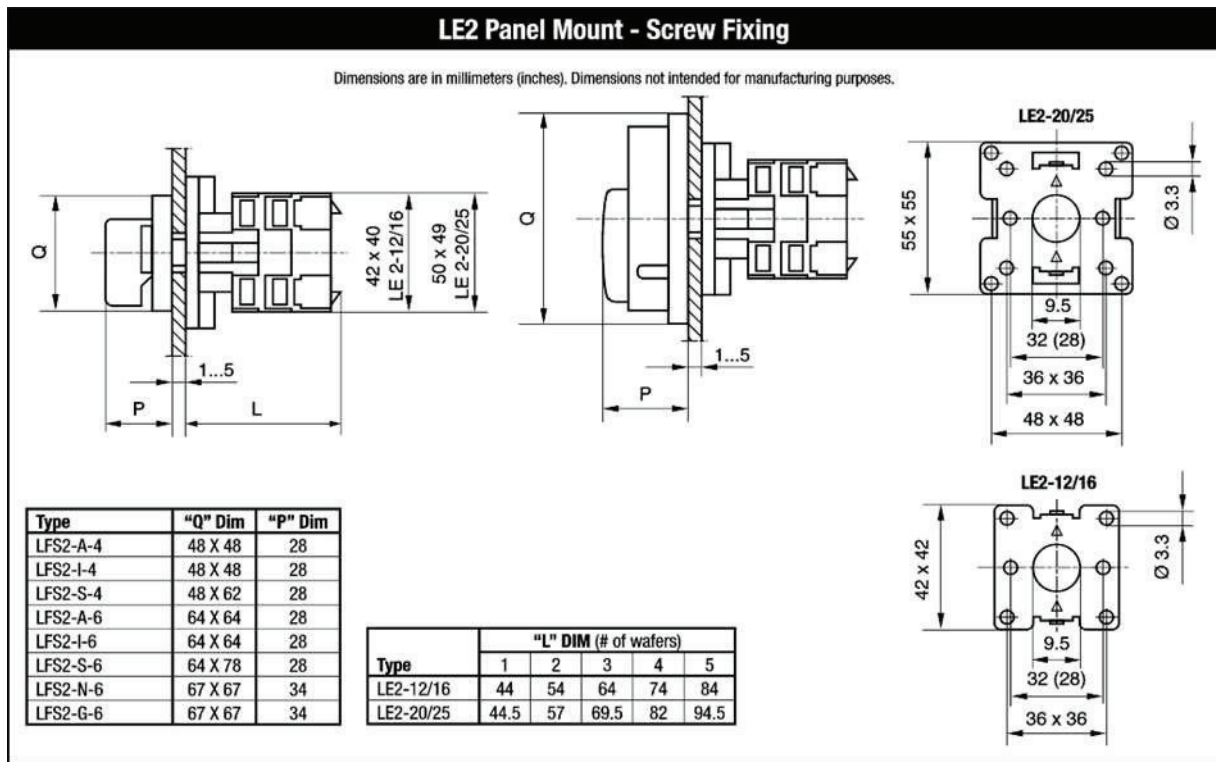
Dimension Diagram
