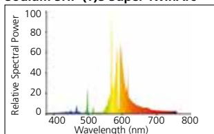
Sodium SHP-(T)S Super TwinArc
