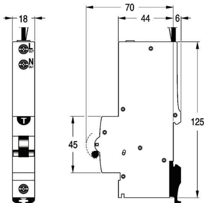
Dimension Diagram
