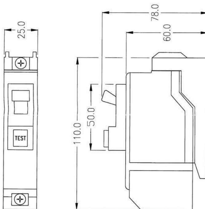
Dimension Diagram
