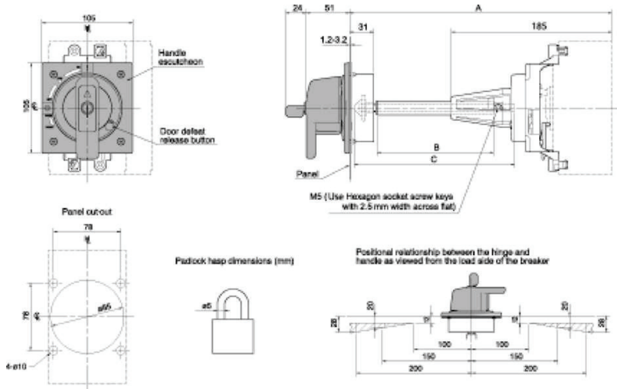
Dimension Diagram
