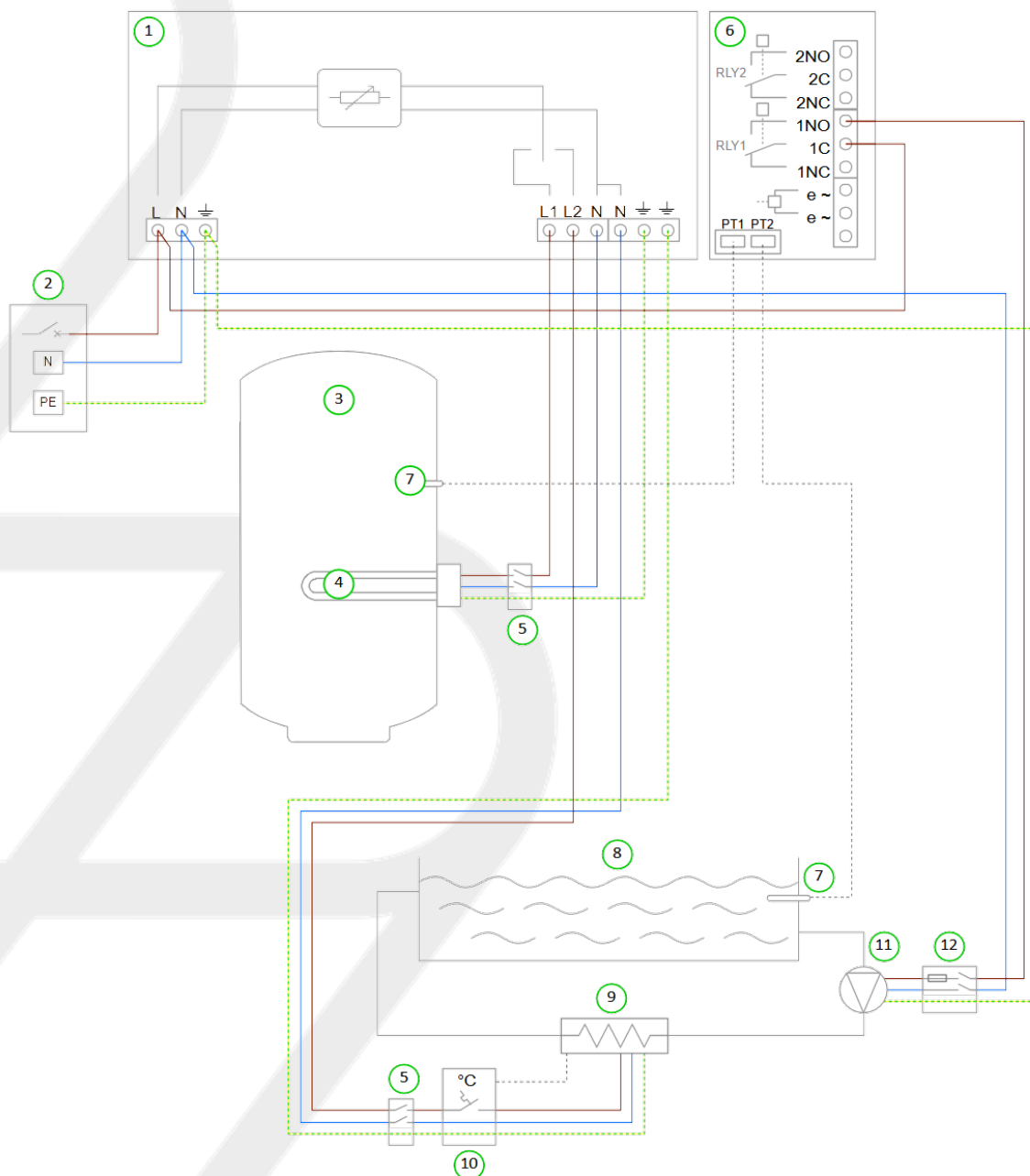
Key for Wiring Diagram 14
