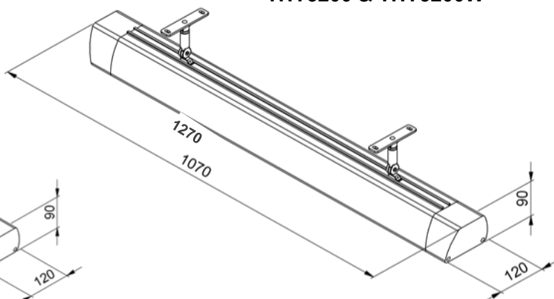
THY3200 & THY3200W
