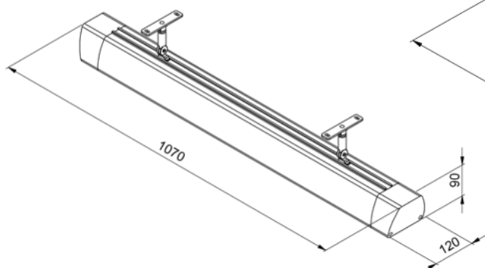
THY2200 & THY2200W
